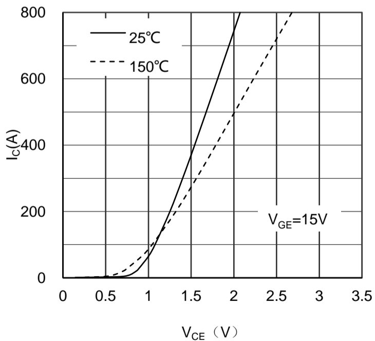
Figure 1. Typical Output Characteristics IGBT-inverter
