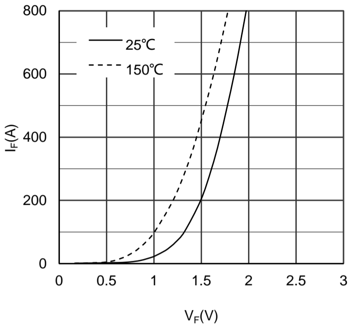
Figure 9. Diode Forward Characteristics Diode -inverter
