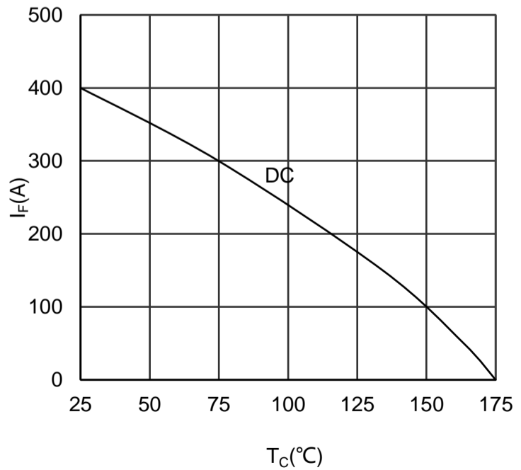
Figure 8. Forward current vs Case temperature Diode-inverter
