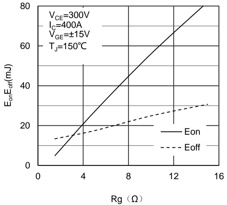
Figure 4. Switching Energy vs Gate Resistor IGBT-inverter
