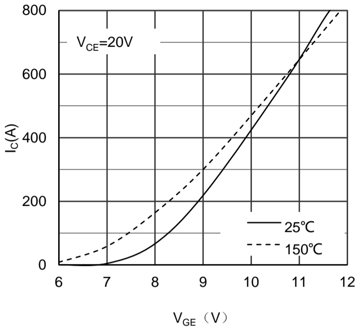
Figure 3. Typical Transfer characteristics IGBT-inverter
