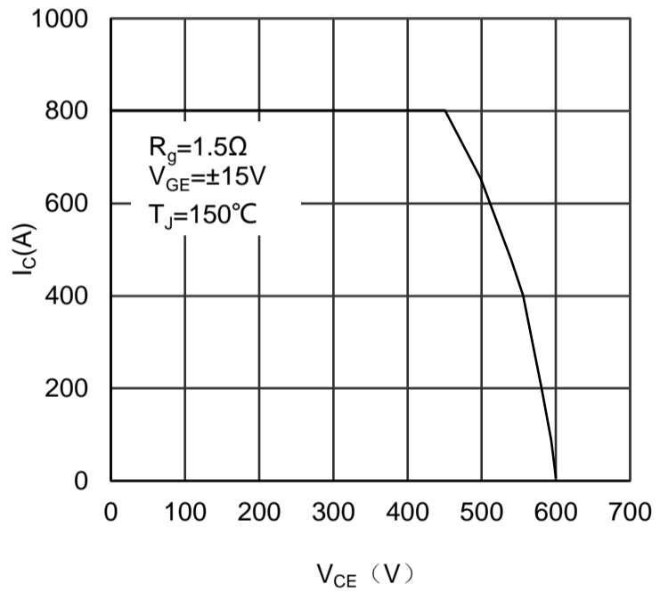
Figure 6. Reverse Bias Safe Operating Area IGBT-inverter
