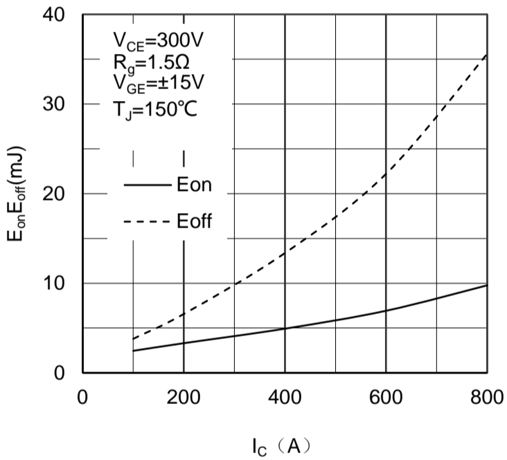
Figure 5. Switching Energy vs Collector Current IGBT-inverter
