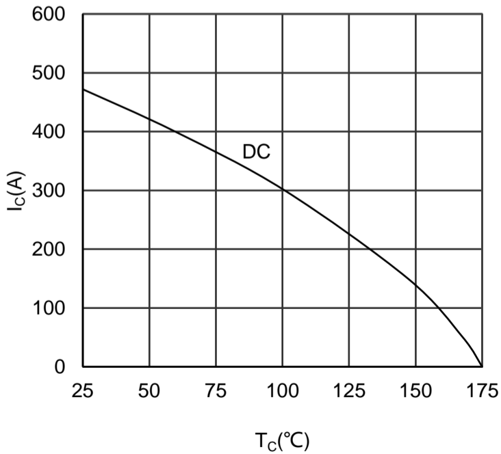
Figure 7. Collector Current vs Case temperature IGBT-inverter
