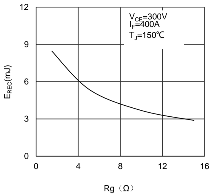
Figure 10. Switching Energy vs Gate Resistor Diode -inverter
