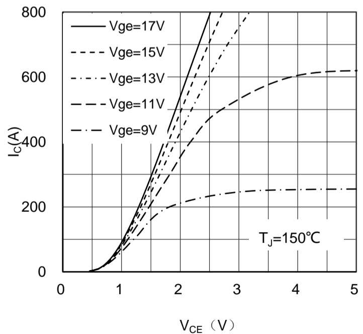
Figure 2. Typical Output Characteristics IGBT-inverter
