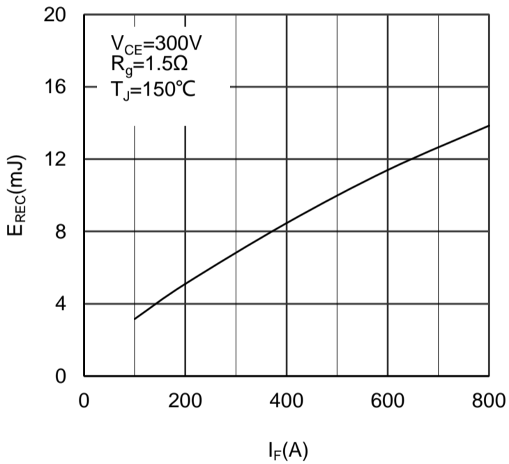
Figure 11. Switching Energy vs Forward Current Diode-inverter
